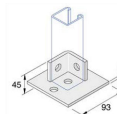
SINGLE CHANNEL BASE PLATE
