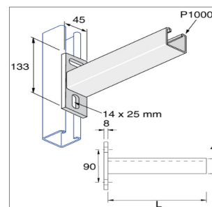
CANTILEVER WALL BRACKET 750mm
