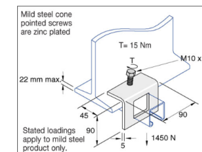
WINDOW CLAMP 41x41 mm
