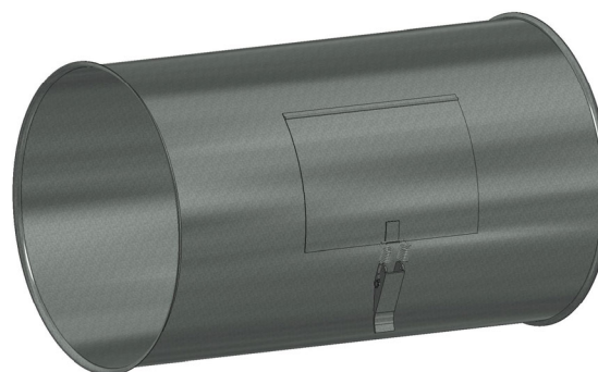
HINGED ACCESS DOOR ON 0.5M STRAIGHT DUCTING
