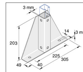
FLOOR PLATE 203 x 305mm
