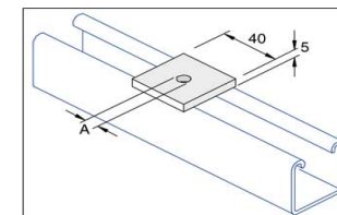
SQUARE WASHER 41x41mm A= 8 & 10mm
