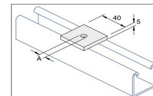
SQUARE WASHER 41x41mm A= 8 & 10mm
