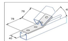
45° ANGLE BRACKET Also in 30° & 60°
